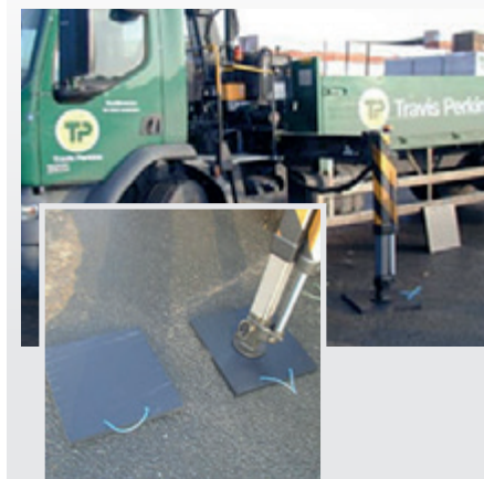
GTf-CRANEPAD500 Crane Pads GT Factors
